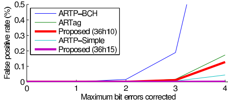
Fig. 7. Empirical false positives. The best performing methods, in terms of the rate of false positives on the LabelMe dataset, are 36h15 and ARTToolkitPlus-Simple. These two coding families also have the fewest number of distinguishable codes, which gives them an advantage. The other three systems have approximately comparable numbers of distinguishable codes; ARTToolkitPlus-BCH performs very poorly; ARTag does much better, and our proposed 36h10 encoding does even better.
